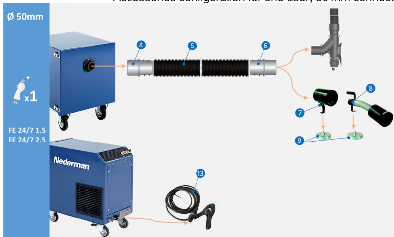
Accessories configuration for one user, 50 mm connection:
