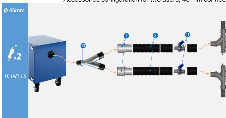
Accessories configuration for two users, 45 mm connection:
