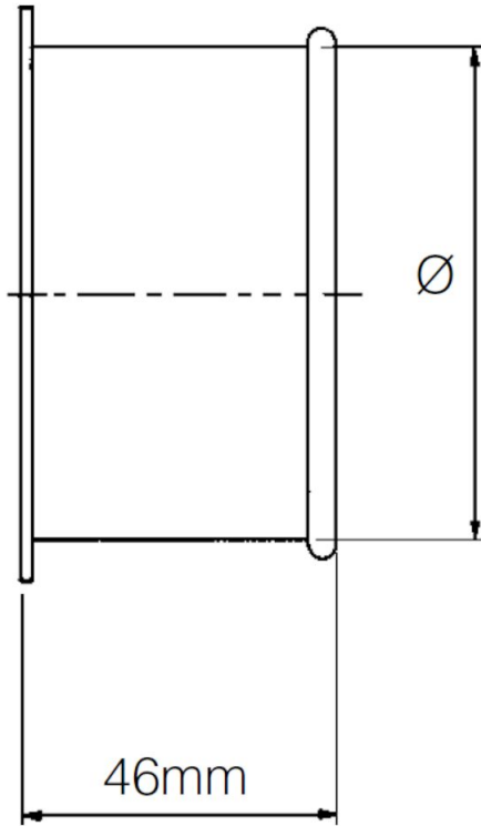
QF Tabular rivet adapter dimensions
