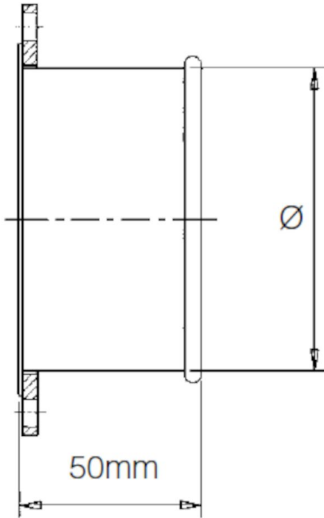
QF Flanged adapter dimensions
