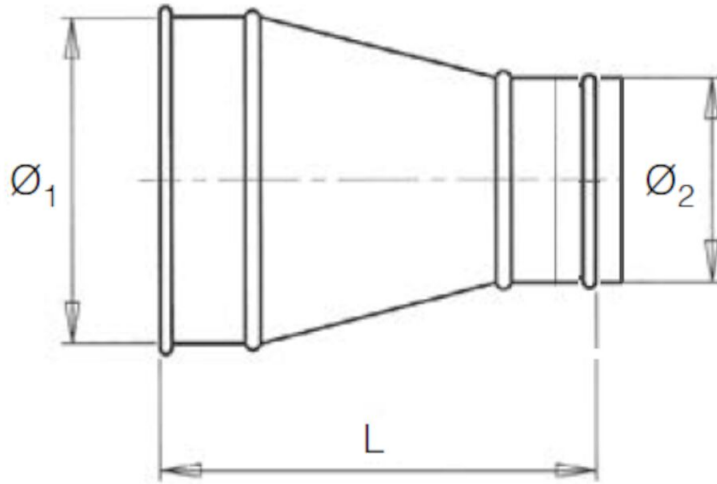
QF Cone for hose connection dimensions
