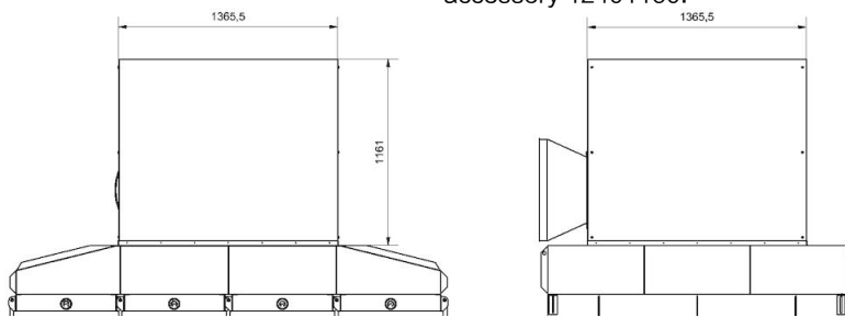
Dimension Fan Enclosure OSF4x3000_OMF2x6000, accessory 12401160:
