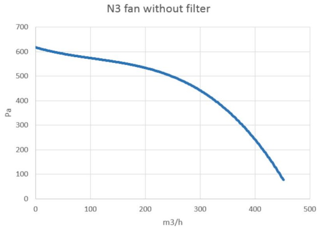
Pressure diagram
