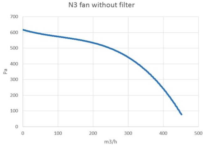
Pressure diagram
