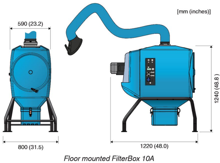
FilterBox 10A Floor
